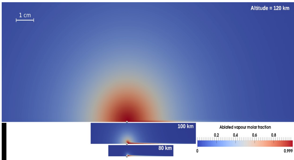
Fields for the ablated vapour molar fraction for three different altitudes of detection: 80, 100, and 120 km. The wall temperature is 2000 K, the diameter of the body 1 mm, and its velocity 32 km/s. The freestream flows from left to right.
